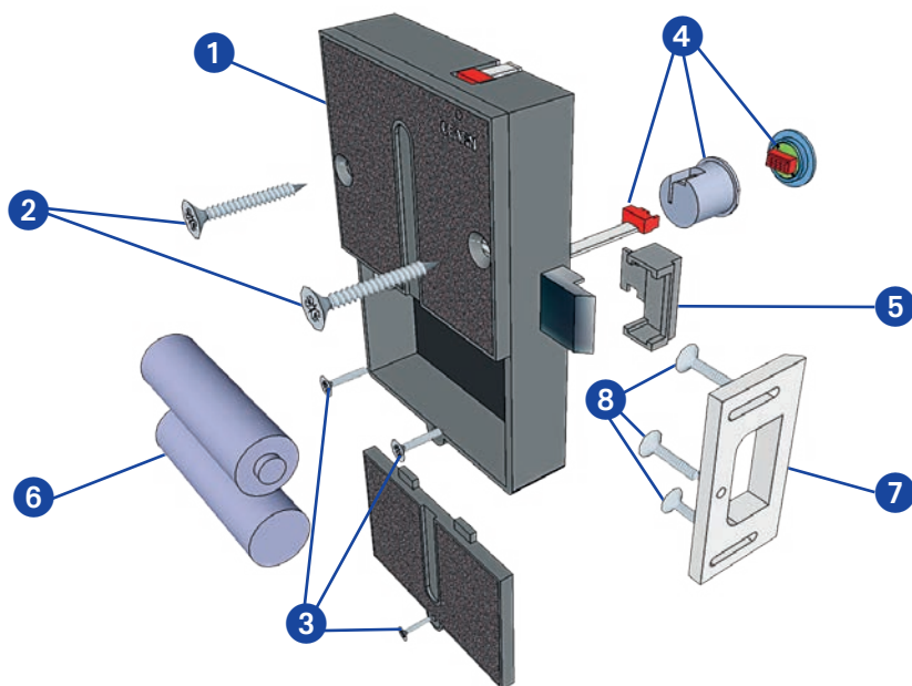
1 M400 SV Furniture lock
